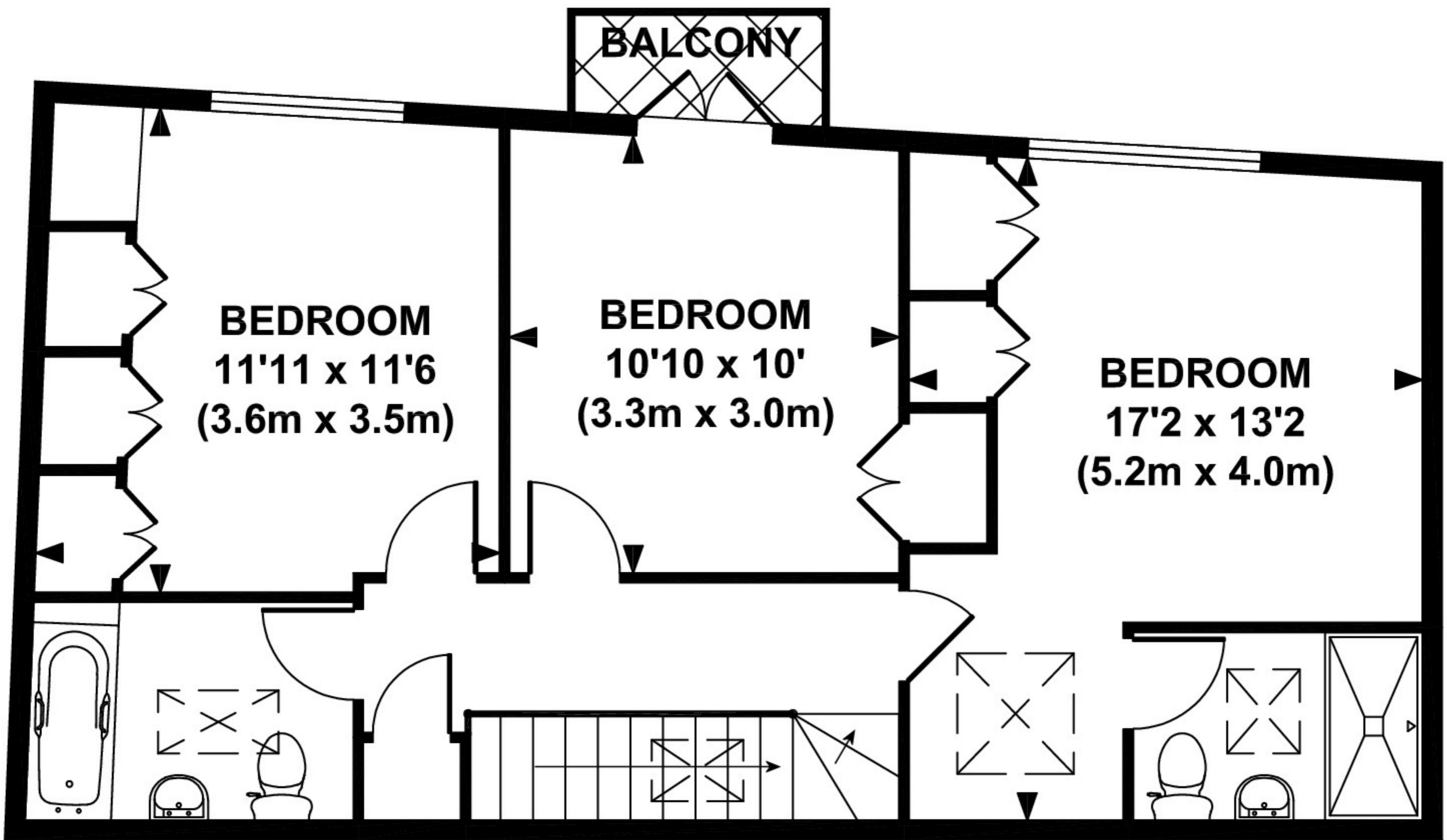
FIRST FLOOR GROSS INTERNAL FLOOR AREA 608 SQ FT
