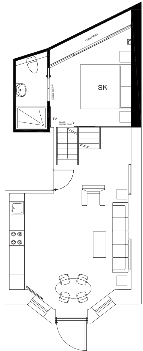
FRONT UPPER MEZZANINE FLOOR
